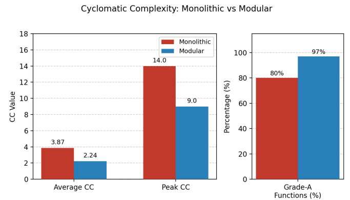
Fig. 3. Cyclomatic Complexity Comparison: Monolithic vs Modular
