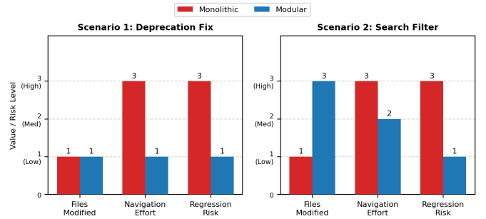
Fig. 4. Change Impact Comparison: Files Modified, Navigation Effort, and Regression Risk (1 = Low, 3 = High) across two controlled modification scenarios
